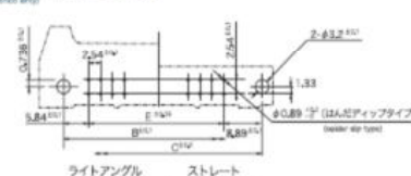
● プリント板レイアウト (参考図) [TOP VIEW] Print board layout (Reference drawing) [TOP VIEW]
